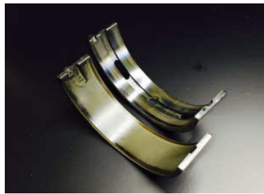
High load capacity main bearing improves the durability under high torque.
